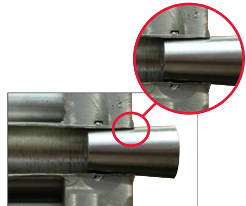
Limited contact with tube/tubesheet
