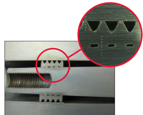
Multiple points of contact with tube/tubesheet
